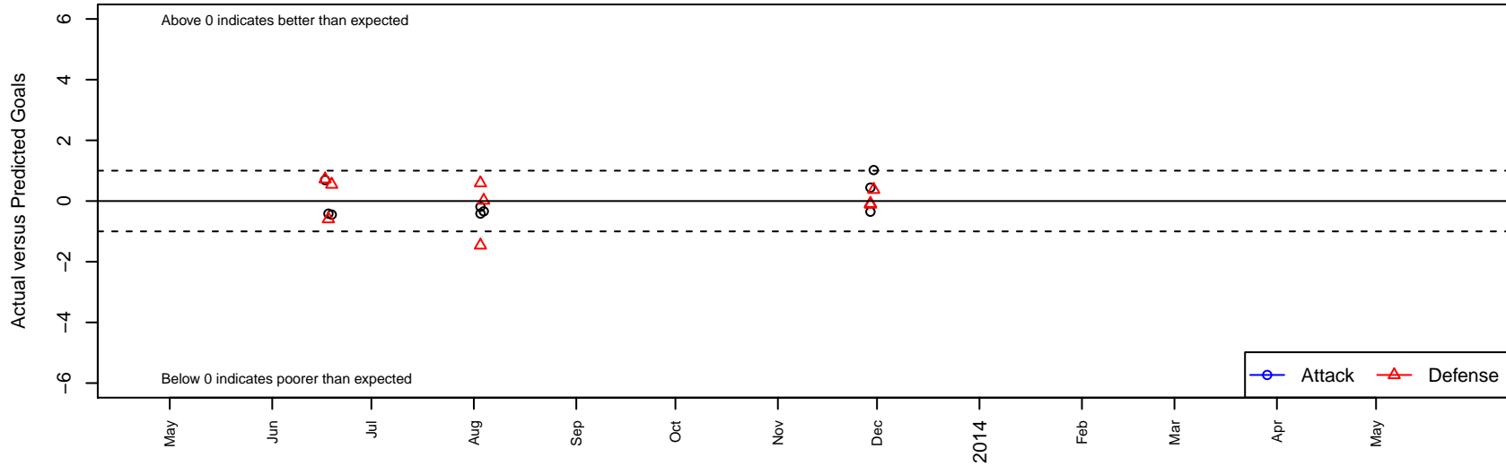
Sparta United 01 Premier TM G00 Dots are actual minus expected GF (blue circles) and GA (red triangles). Blue line is smoothed change in attack strength. Red is smoothed change in defense strength.
